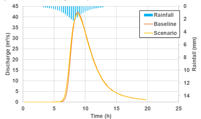
Figure 2: Comparison of the model outputs for the baseline model and the cross slope tree planting scenario
