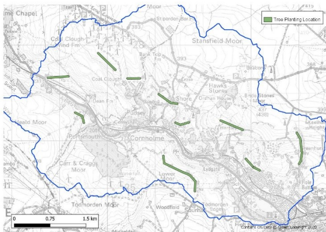
Figure 1: Map of modelled cross slope tree planting locations for the Calder upstream of Todmorden
